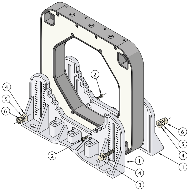
Right angle brackets mounting on NCS165T sensors
