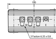
Size 1 - CS500BR and CS1000BR and HRS1000-T-003/T-004 and HRS1500-T-003/T-004
