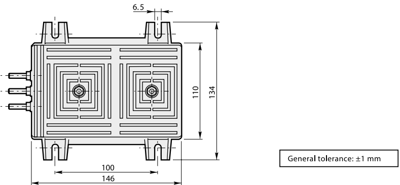
Size 1 (VS2000B to VS4200B)
