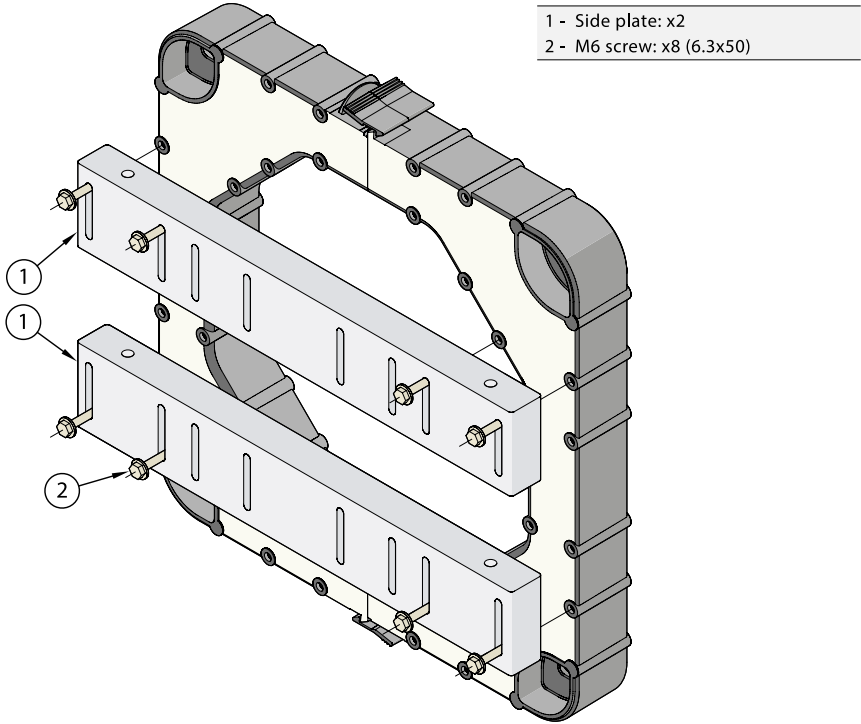
Side plate mounting on NCS305 sensors
