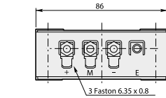
Size 0 - CS300BR and CS503BR
