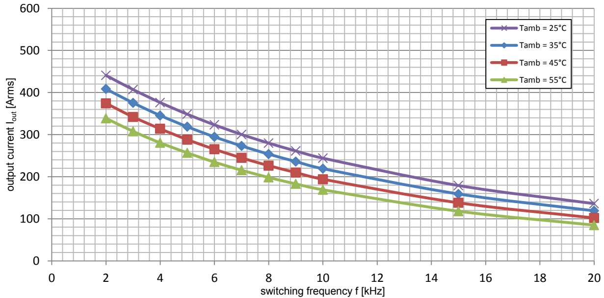
Figure 5: Current rating VARIS™-06-12-A (3-phase), Measurement at V_{dc}=600\text{V} , v_{air} = 6\text{m/s} , V_{ac}=400\text{Vrms} , \cos(\varphi)=0.95 , m=1.0 , f_{ac\_sine}=50\text{Hz} , T_{vjsw}\leq 125^\circ\text{C}
