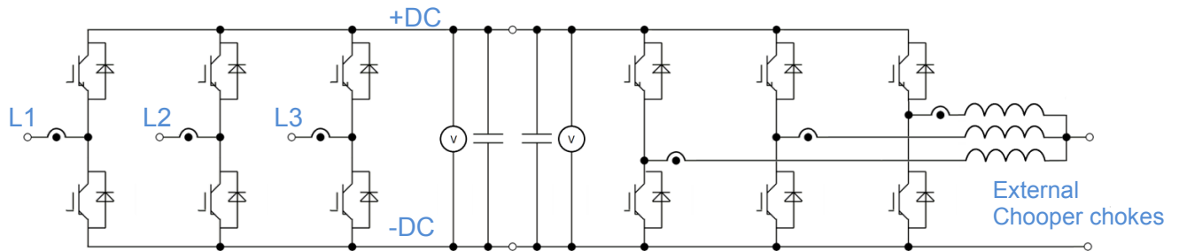
Figure 3: 3-phase AFE with triple interleaved Chopper
