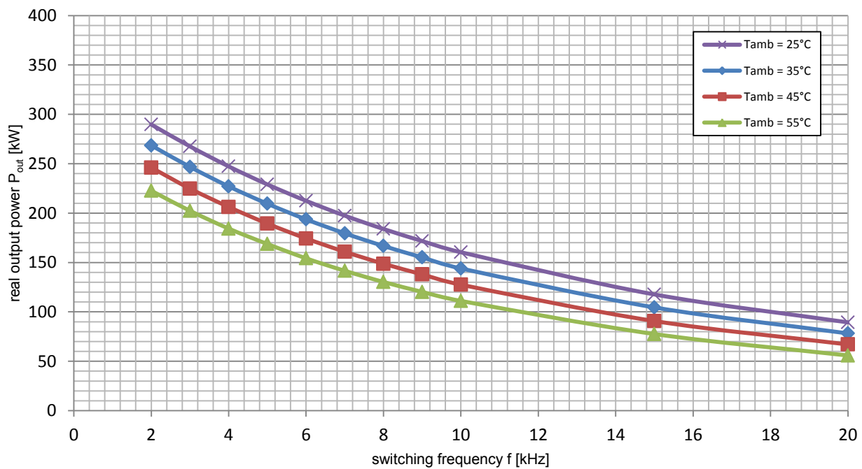
Figure 6: Power rating VARIS™-06-12-A (3-phase) Measurement at V_{dc}=600\text{V} , v_{air} = 6\text{m/s} , V_{ac}=400\text{Vrms} , \cos(\varphi)=0.95 , m=1.0 , f_{ac\_sine}=50\text{Hz} , T_{vjsw}\leq 125^\circ\text{C}
