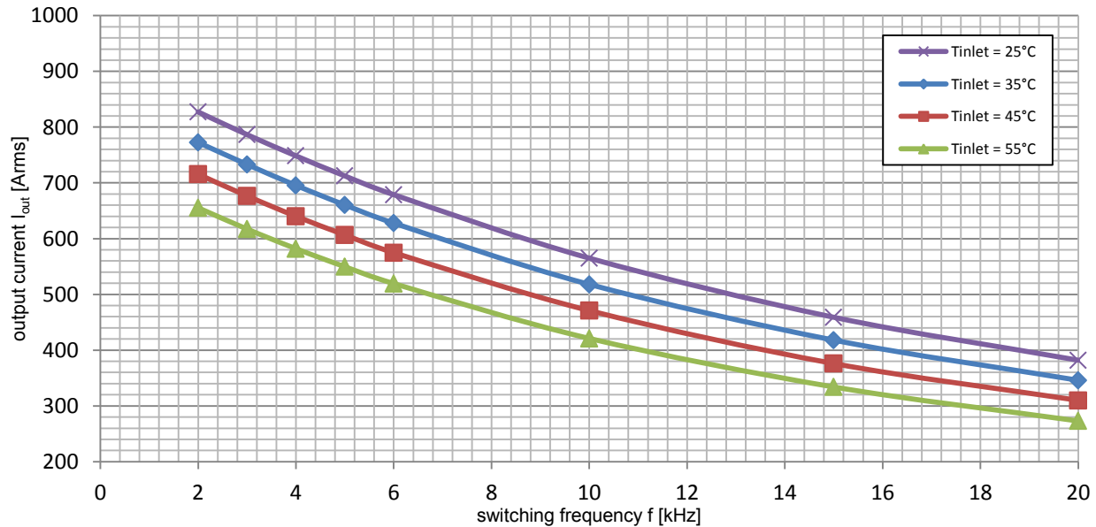
Figure 7: Current rating VARIS™-06-12-W (3-phase, water cooled) Measurement at V_{dc}=600\text{V} , Q = 4,3 \text{ L/min} , V_{ac}=400\text{Vrms} , \cos(\varphi)=0.95 , m=1.0 , f_{ac\_sine}=50\text{Hz} , T_{vjsw}\leq 125^{\circ}\text{C}
