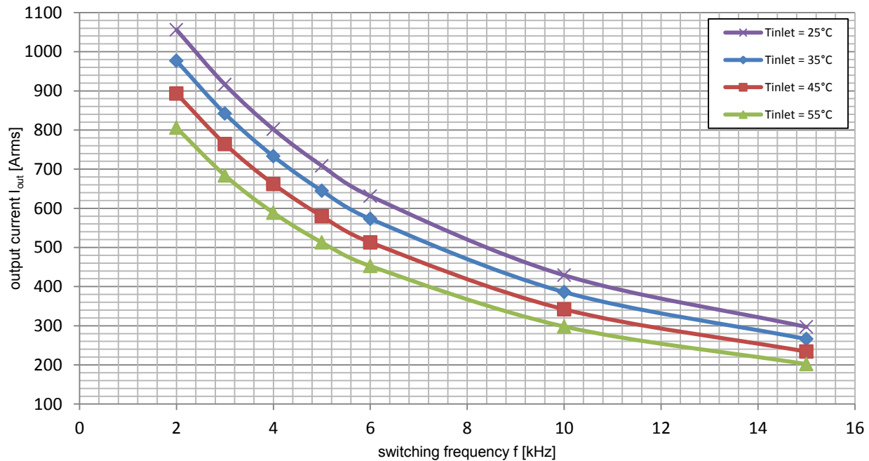
Figure 7: Current rating VARIS™-10-17-W (3-phase, water cooled) Measurement at V_{dc}=1000\text{V} , Q = 4,3 \text{ L/min} , V_{ac}=690\text{V}_{\text{RMS}} , \cos(\varphi)=0.95 , m=1.0 , f_{ac\_sine}=50\text{Hz} , T_{vjsw} \leq 125^{\circ}\text{C}
