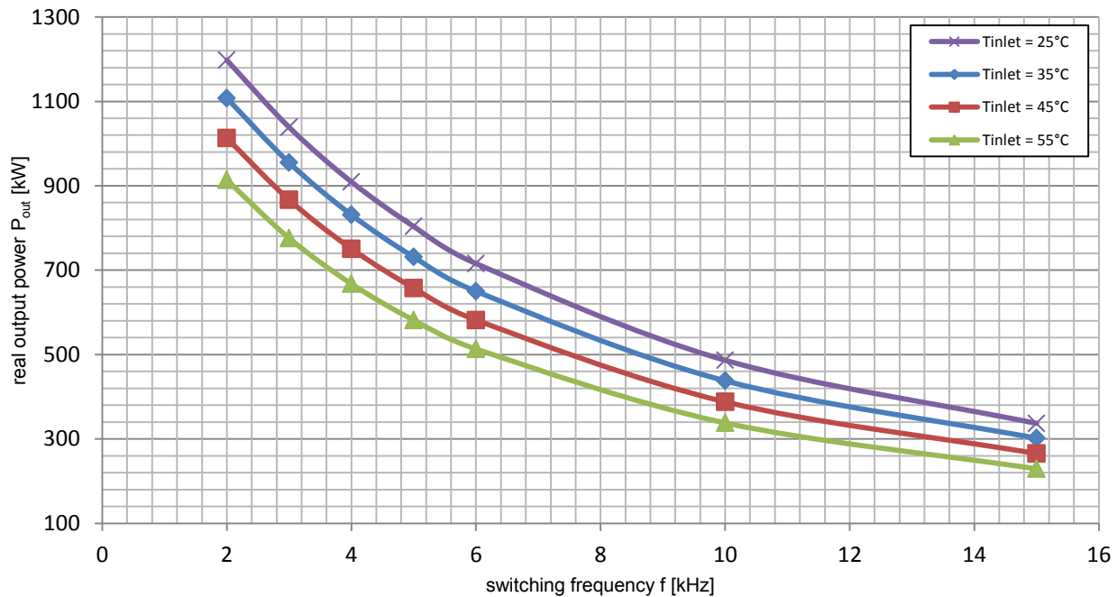
Figure 8: Power rating VARIS™-10-17-W (3-phase, water cooled) Measurement at V_{dc}=1000\text{V} , Q = 4,3 \text{ L/min} , V_{ac}=690\text{V}_{\text{RMS}} , \cos(\varphi)=0.95 , m=1.0 , f_{ac\_sine}=50\text{Hz} , T_{vjsw} \leq 125^{\circ}\text{C}
