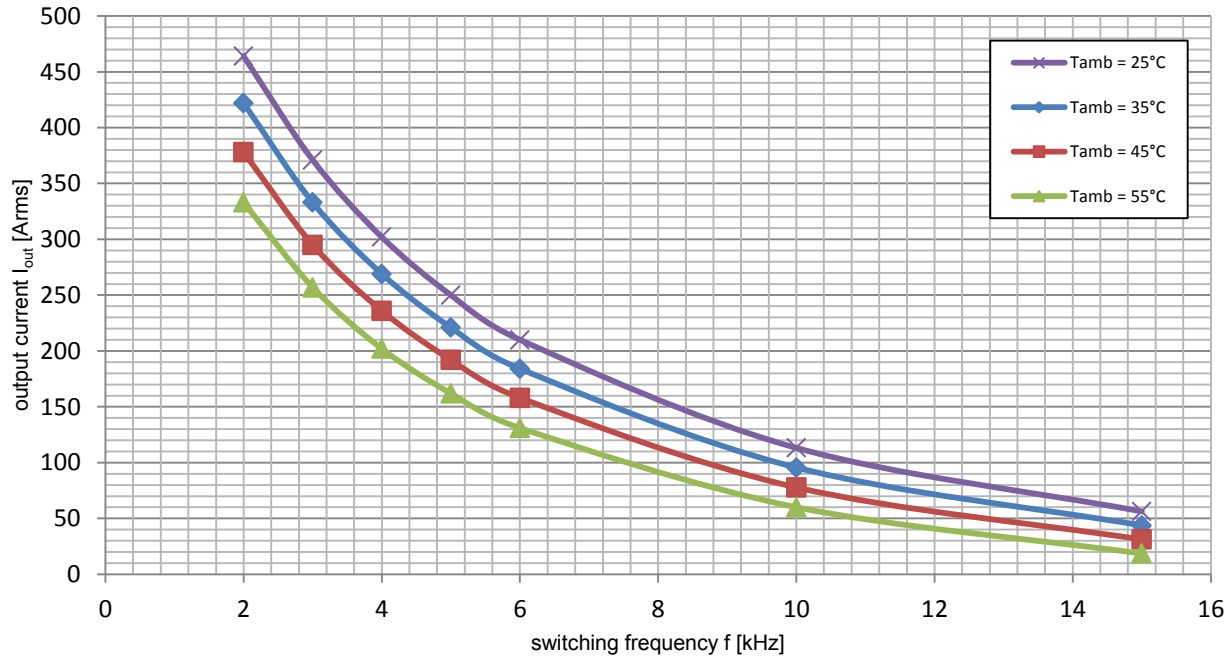
Figure 5: Current rating VARIS™-10-17-A (3-phase), Measurement at V_{dc}=1000\text{V} , v_{air} = 6\text{m/s} , V_{ac}=690\text{VRMS} , \cos(\varphi)=0.95 , m=1.0 , f_{ac\_sine}=50\text{Hz} , T_{vjsw}\leq 125^\circ\text{C}
