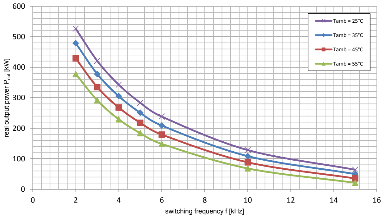
Figure 6: Power rating VARIS™-10-17-A (3-phase) Measurement at V_{dc}=1000\text{V} , v_{air} = 6\text{m/s} , V_{ac}=690\text{VRMS} , \cos(\varphi)=0.95 , m=1.0 , f_{ac\_sine}=50\text{Hz} , T_{vjsw}\leq 125^\circ\text{C}
