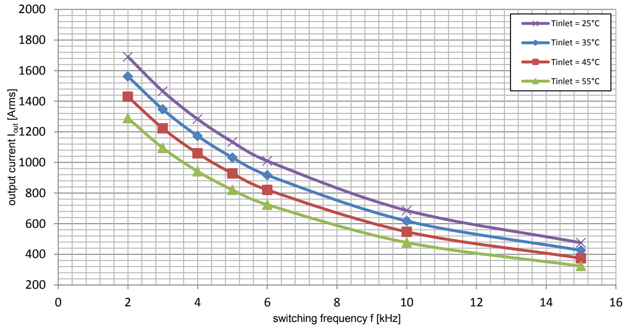
Figure 12: Current rating VARIS™ XT-10-17 (3-phase configuration, paralleled modules) Measurement at V_{dc}=1000\text{V} , Q = 12 \text{ L/min} , V_{ac}=690\text{V}_{\text{RMS}} , \cos(\varphi)=0.95 , m=1.0 , f_{ac\_sine}=50\text{Hz} , T_{vjsw}\leq 125^{\circ}\text{C}
