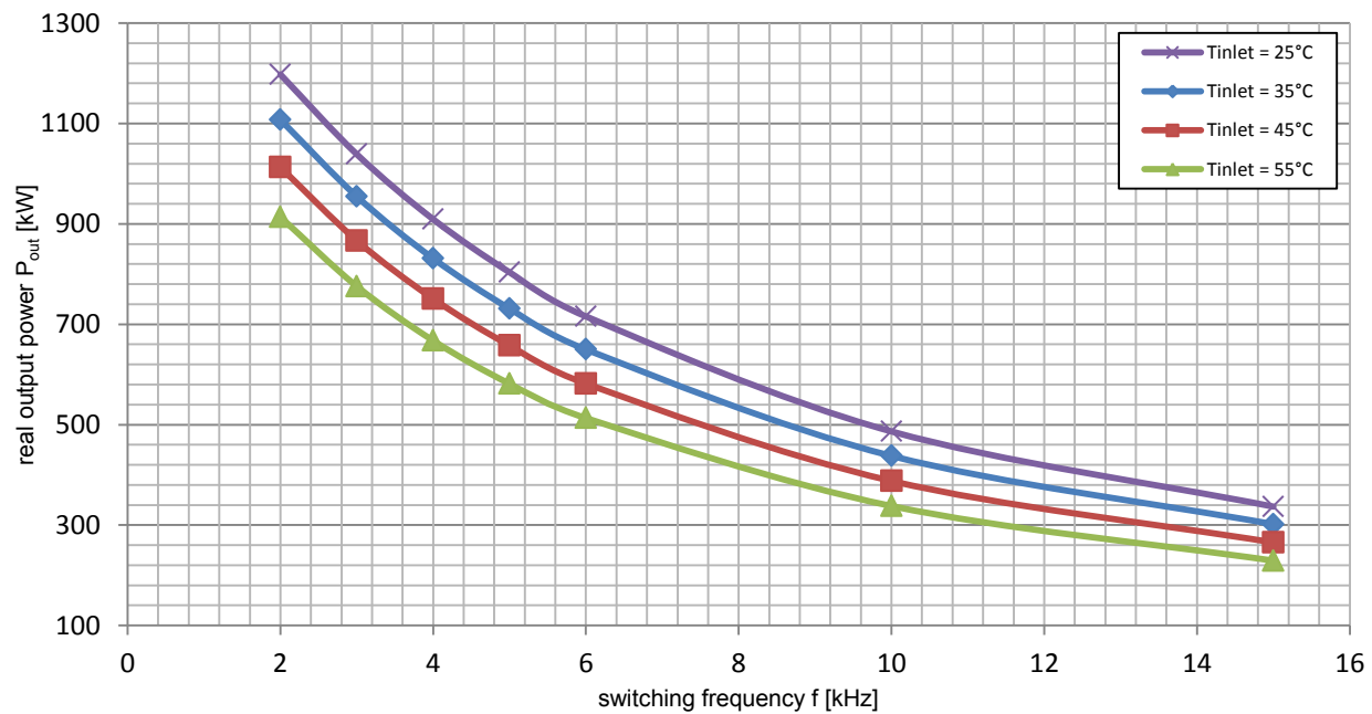
Figure 11: Power rating VARIS™ XT-10-17 (3-phase configuration) Measurement at V_{dc}=1000\text{V} , Q = 12 \text{ L/min} , V_{ac}=690\text{V}_{\text{RMS}} , \cos(\varphi)=0.95 , m=1.0 , f_{ac\_sine}=50\text{Hz} , T_{vjsw}\leq 125^{\circ}\text{C}
