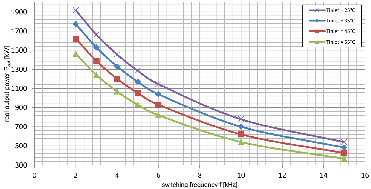
Figure 13: Power rating VARIS™ XT-10-17 (3-phase configuration, paralleled modules) Measurement at V_{dc}=1000\text{V} , Q = 12 \text{ L/min} , V_{ac}=690\text{V}_{\text{RMS}} , \cos(\varphi)=0.95 , m=1.0 , f_{ac\_sine}=50\text{Hz} , T_{vjsw}\leq 125^{\circ}\text{C}
