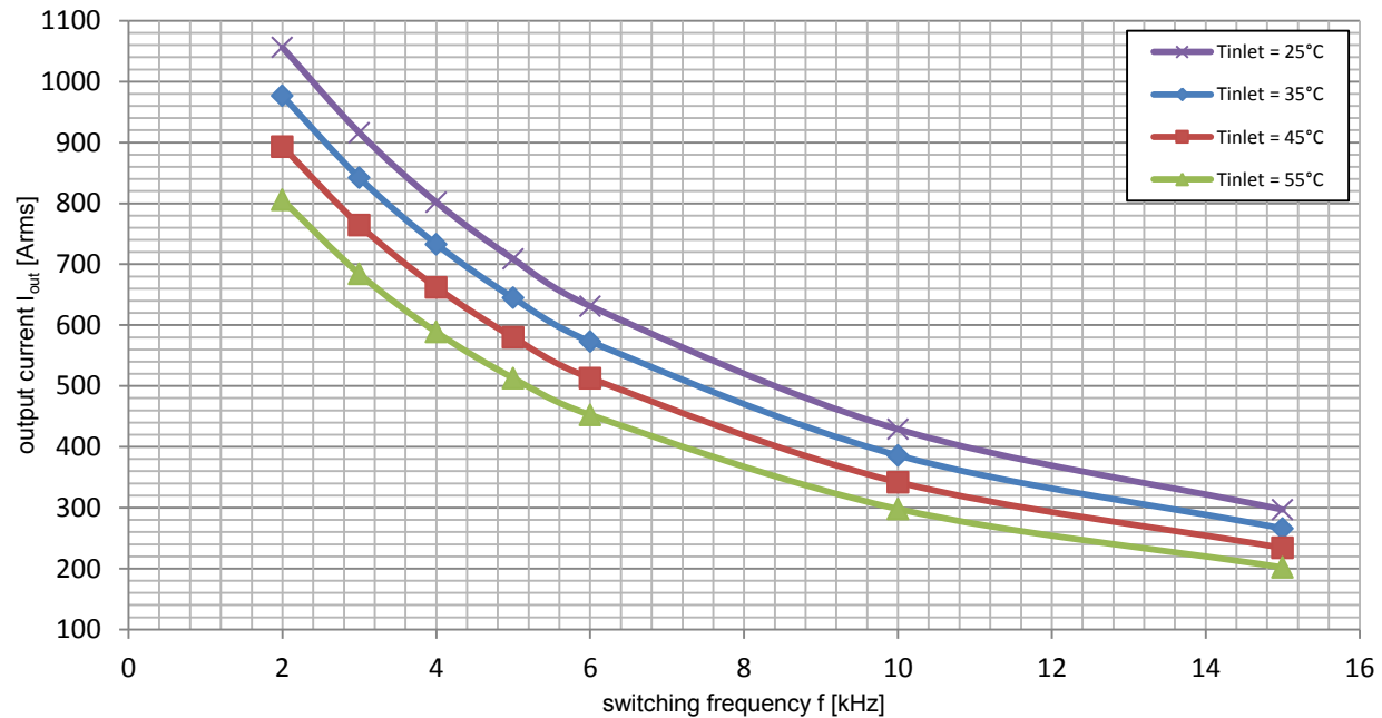
Figure 10: Current rating VARIS™ XT-10-17 (3-phase configuration) Measurement at V_{dc}=1000\text{V} , Q = 12 \text{ L/min} , V_{ac}=690\text{V}_{\text{RMS}} , \cos(\varphi)=0.95 , m=1.0 , f_{ac\_sine}=50\text{Hz} , T_{vjsw}\leq 125^{\circ}\text{C}
