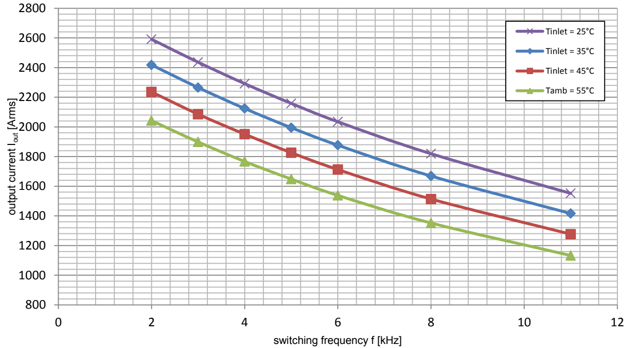
Figure 12: Current rating VARIS™ XT-14-12 (3-phase configuration, paralleled modules) Measurement at V_{dc}=600\text{V} , Q = 12 \text{ L/min} , V_{ac}=400\text{V}_{\text{RMS}} , \cos(\phi)=0.95 , m=1.0 , f_{ac\_sine}=50\text{Hz} , T_{vjsw}\leq 125^{\circ}\text{C}
