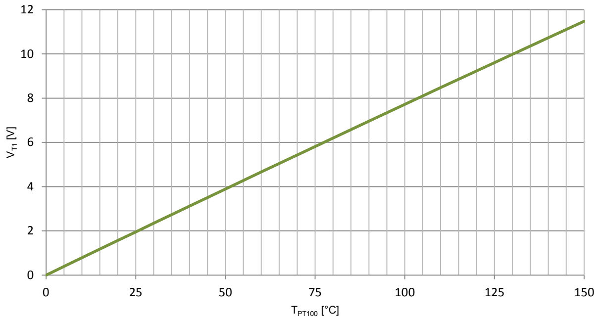
Figure 8: Characteristic curve of the analog heatsink temperature V_{T1} over the PT100 temperature sensor
