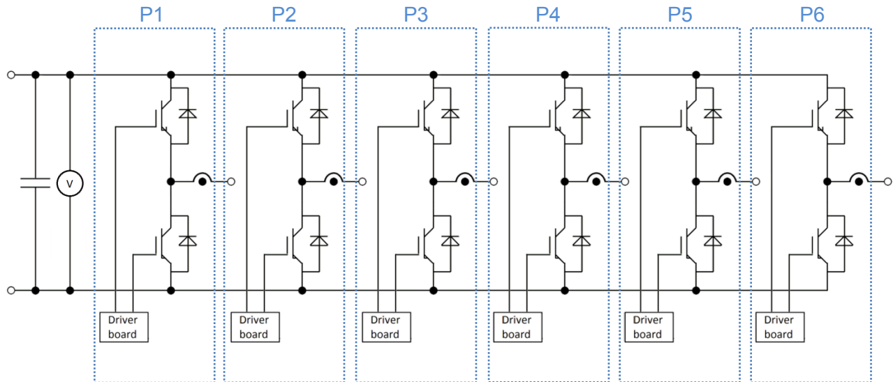
Figure 1: Standard hardware setup
