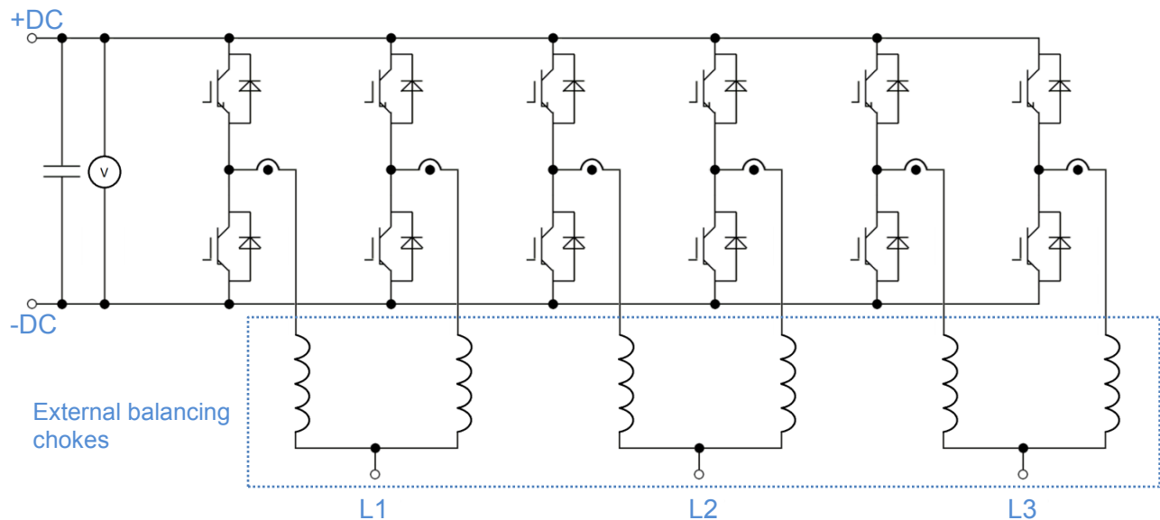
Figure 5: Soft paralleling of the AC- output/input with external balancing chokes
