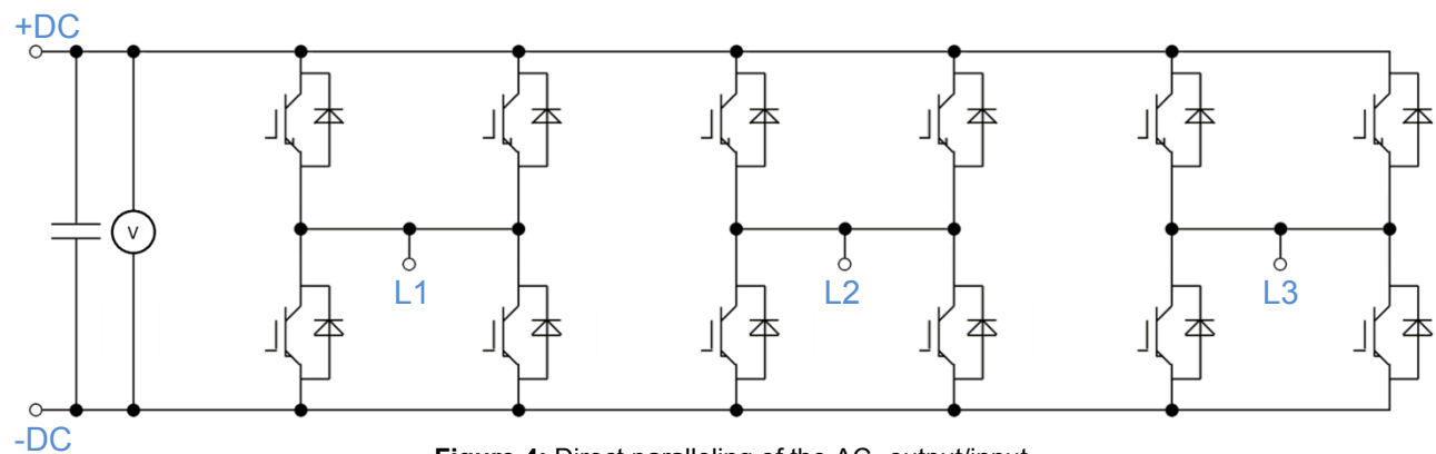
Figure 4: Direct paralleling of the AC- output/input
