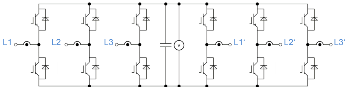
Figure 2: Frequency or Back-to-Back Inverter
