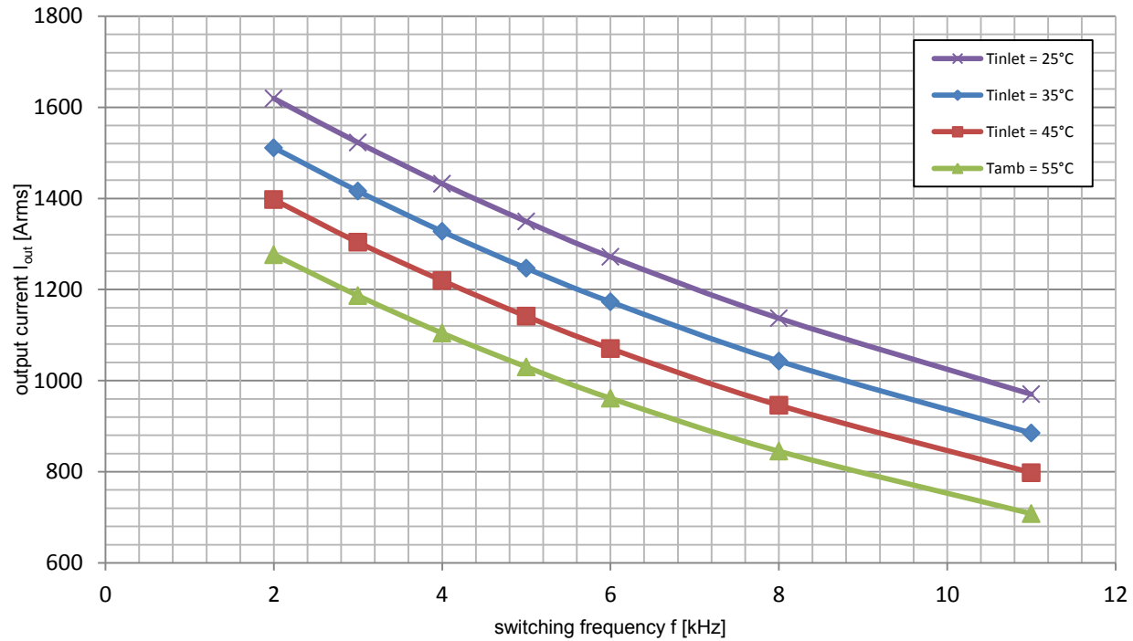
Figure 10: Current rating VARIS™ XT-14-12 (3-phase configuration) Measurement at V_{dc}=600V , Q = 12 \text{ L/min} , V_{ac}=400V_{RMS} , \cos(\varphi)=0.95 , m=1.0 , f_{ac\_sine}=50Hz , T_{vjsw} \leq 125^\circ C
