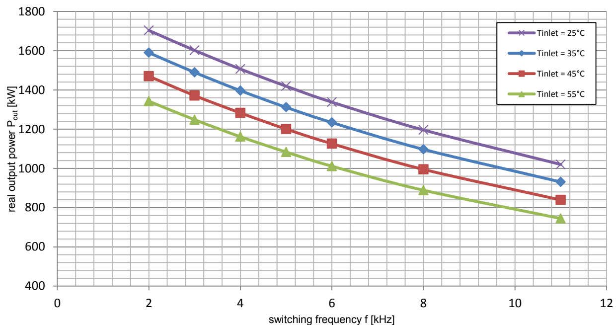
Figure 13: Power rating VARIS™ XT-14-12 (3-phase configuration, paralleled modules) Measurement at V_{dc}=600\text{V} , Q = 12 \text{ L/min} , V_{ac}=400\text{V}_{\text{RMS}} , \cos(\phi)=0.95 , m=1.0 , f_{ac\_sine}=50\text{Hz} , T_{vjsw}\leq 125^{\circ}\text{C}
