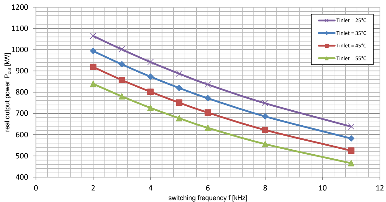
Figure 11: Power rating VARIS™ XT-14-12 (3-phase configuration) Measurement at V_{dc}=600V , Q = 12 \text{ L/min} , V_{ac}=400V_{RMS} , \cos(\varphi)=0.95 , m=1.0 , f_{ac\_sine}=50Hz , T_{vjsw} \leq 125^\circ C
