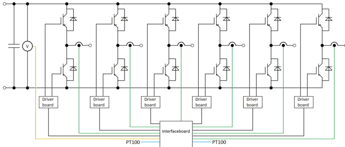
Figure 6: VARIS™ XT circuit arrangement with Interfaceboard
