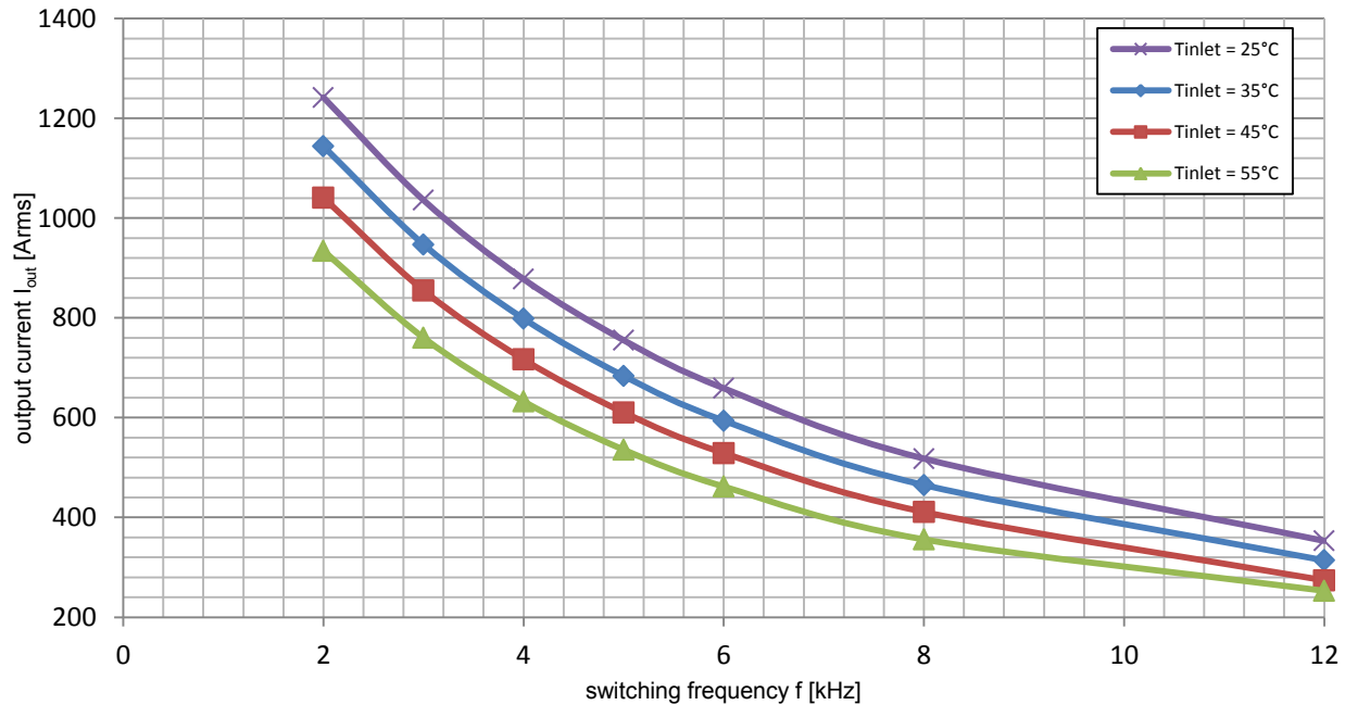
Figure 10: Current rating VARIS™ XT-14-17 (3-phase configuration) Measurement at V_{dc}=1000\text{V} , Q = 12 \text{ L/min} , V_{ac}=690\text{V}_{\text{RMS}} , \cos(\varphi)=0.95 , m=1.0 , f_{ac\_sine}=50\text{Hz} , T_{vjsw}\leq 125^{\circ}\text{C}
