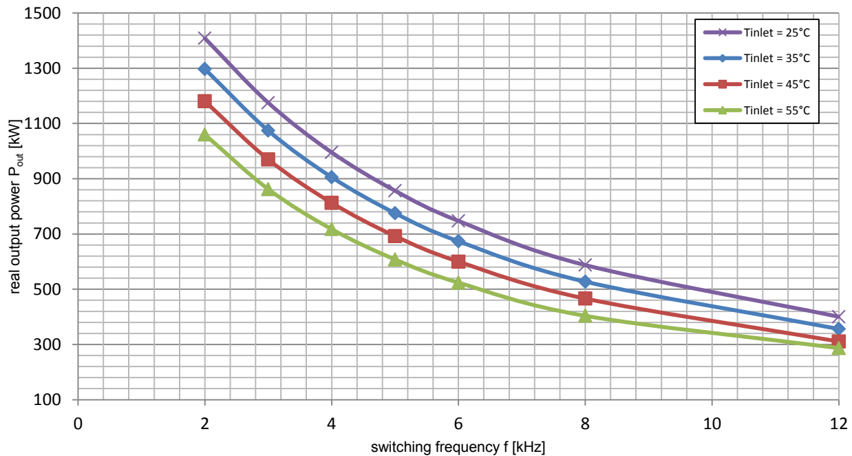
Figure 11: Power rating VARIS™ XT-14-17 (3-phase configuration) Measurement at V_{dc}=1000\text{V} , Q = 12 \text{ L/min} , V_{ac}=690\text{V}_{\text{RMS}} , \cos(\varphi)=0.95 , m=1.0 , f_{ac\_sine}=50\text{Hz} , T_{vjsw}\leq 125^{\circ}\text{C}
