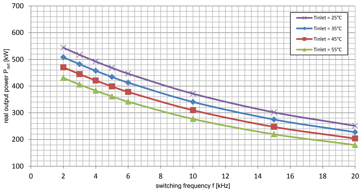
Figure 11: Power rating VARIS™ XT Compact-06-12-W (3-phase, water cooled) Measurement at V_{dc}=600\text{V} , Q = 4,3 \text{ L/min} , V_{ac}=400\text{Vrms} , \cos(\varphi)=0.95 , m=1.0 , f_{ac\_sine}=50\text{Hz} , T_{vjsw}\leq 125^{\circ}\text{C}
