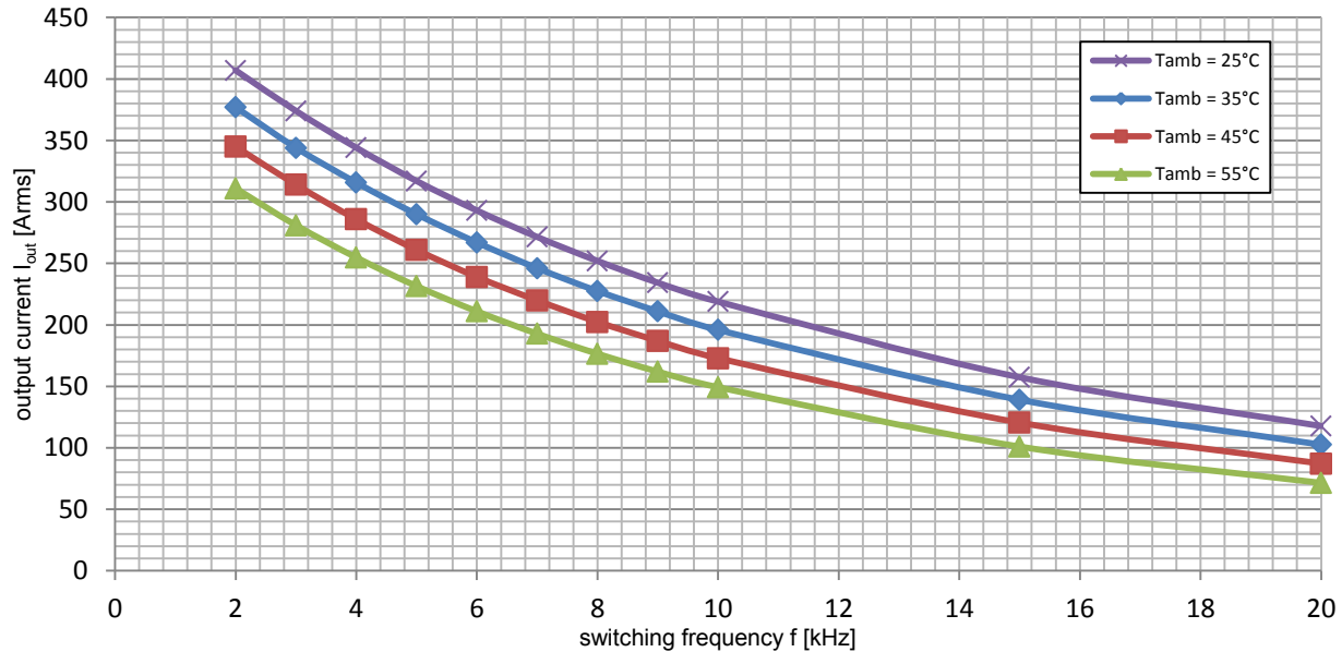
Figure 8: Current rating VARIS™ XT Compact-06-12-A (3-phase), Measurement at V_{dc}=600\text{V} , v_{air} = 6\text{m/s} , V_{ac}=400\text{Vrms} , \cos(\varphi)=0.95 , m=1.0 , f_{ac\_sine}=50\text{Hz} , T_{vjsw}\leq 125^\circ\text{C}
