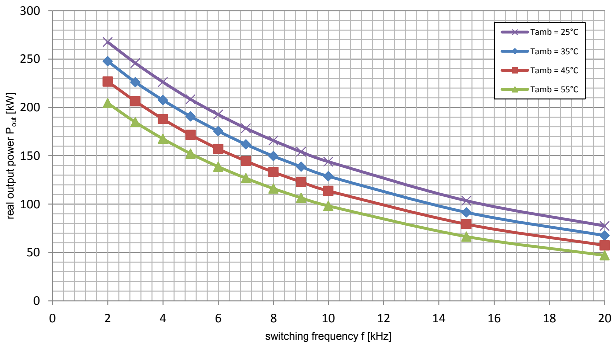
Figure 9: Power rating VARIS™ XT Compact-06-12-A (3-phase) Measurement at V_{dc}=600\text{V} , v_{air} = 6\text{m/s} , V_{ac}=400\text{Vrms} , \cos(\varphi)=0.95 , m=1.0 , f_{ac\_sine}=50\text{Hz} , T_{vjsw}\leq 125^\circ\text{C}
