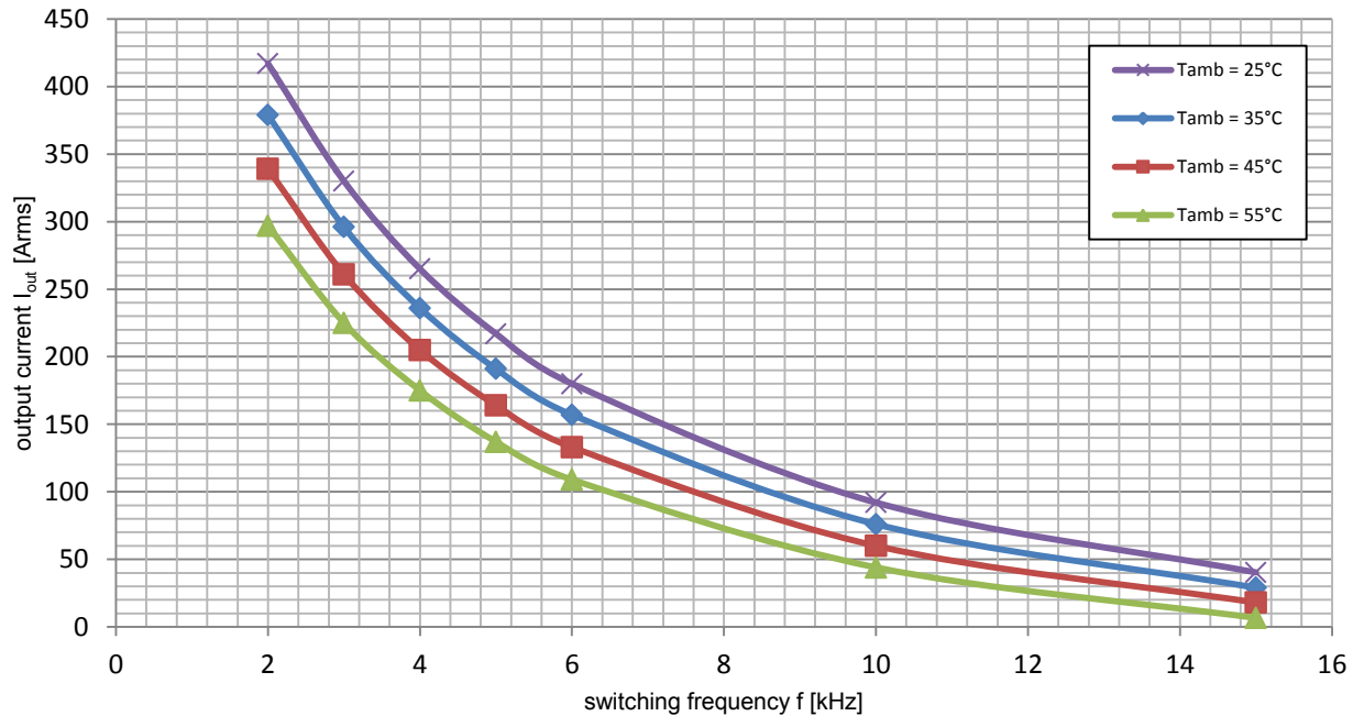
Figure 8: Current rating VARIS™ XT Compact-10-17-A (3-phase), Measurement at V_{dc}=1000\text{V} , v_{air} = 6\text{m/s} , V_{ac}=690\text{VRMS} , \cos(\varphi)=0.95 , m=1.0 , f_{ac\_sine}=50\text{Hz} , T_{vjsw}\leq 125^{\circ}\text{C}
