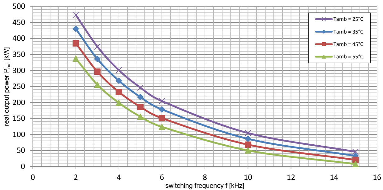
Figure 9: Power rating VARIS™ XT Compact-10-17-A (3-phase) Measurement at V_{dc}=1000\text{V} , v_{air} = 6\text{m/s} , V_{ac}=690\text{VRMS} , \cos(\varphi)=0.95 , m=1.0 , f_{ac\_sine}=50\text{Hz} , T_{vjsw}\leq 125^{\circ}\text{C}
