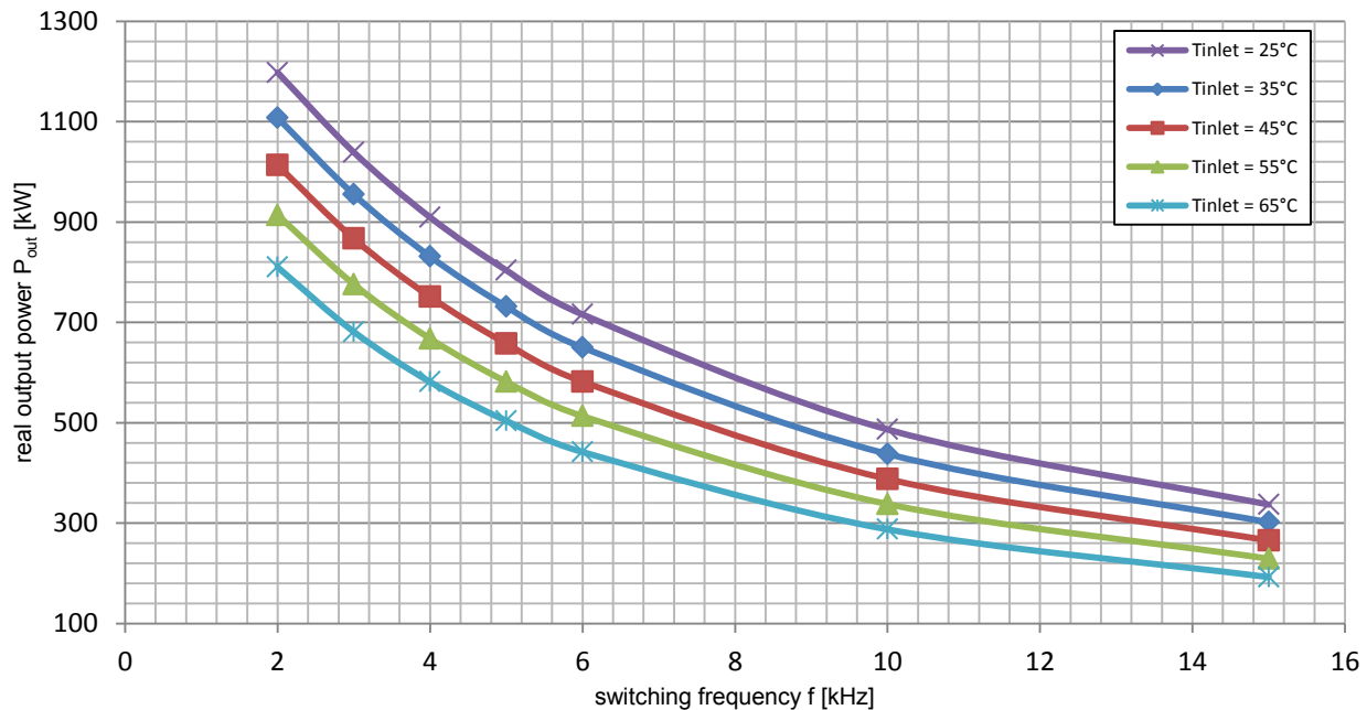
Figure 11: Power rating VARIS™ XT Compact-10-17-W (3-phase, water cooled) Measurement at V_{dc}=1000\text{V} , Q = 4,3 \text{ L/min} , V_{ac}=690\text{V}_{\text{RMS}} , \cos(\varphi)=0.95 , m=1.0 , f_{ac\_sine}=50\text{Hz} , T_{vjsw}\leq 125^\circ\text{C}
