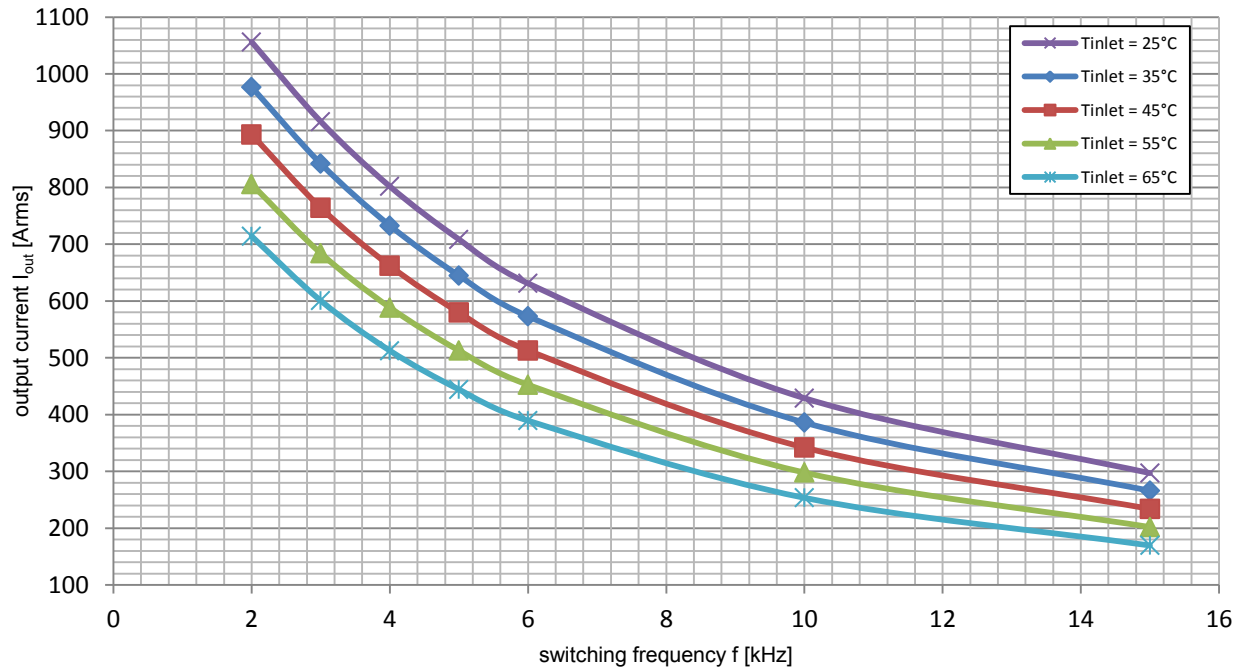
Figure 10: Current rating VARIS™ XT Compact-10-17-W (3-phase, water cooled) Measurement at V_{dc}=1000\text{V} , Q = 4,3 \text{ L/min} , V_{ac}=690\text{V}_{\text{RMS}} , \cos(\varphi)=0.95 , m=1.0 , f_{ac\_sine}=50\text{Hz} , T_{vjsw}\leq 125^\circ\text{C}
